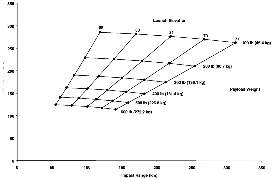
Figure E-16 Taurus-Orion Launch Vehicle Performance
