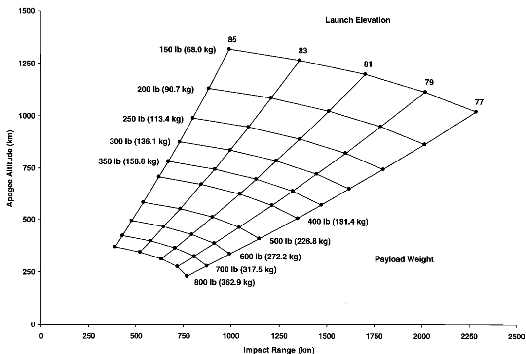
Figure E-18. Black Brant X Launch Vehicle Performance
